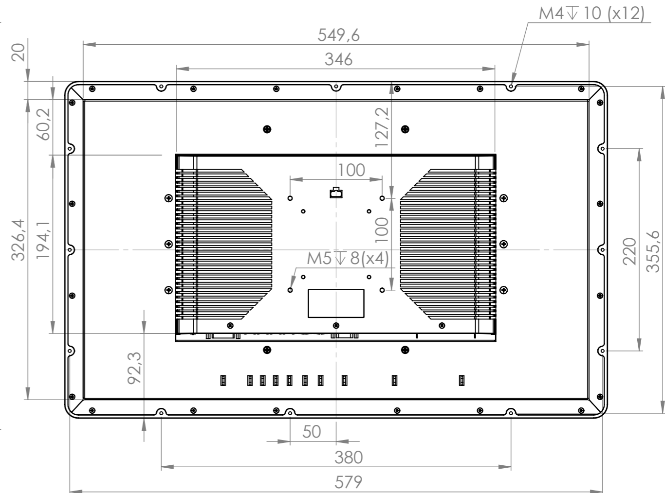
BACK VIEW
