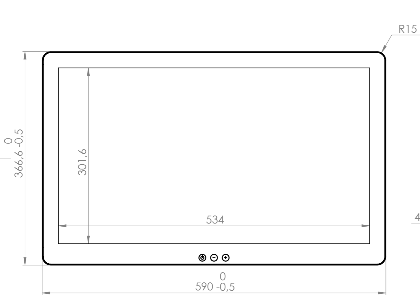
FRONT VIEW
