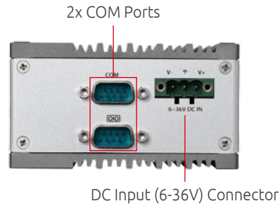
Right side view of MXE-200/200i
